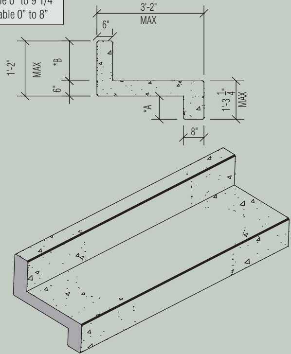
Z-Shape Configuration
